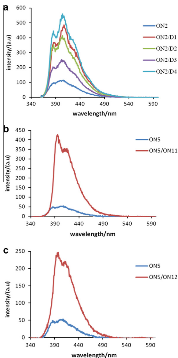
Figure 3. Fluorescence emission spectra of (a) ON2 comprising monomer M upon excitation at 350 nm and pH 6.0 forming parallel triplex and mismatched triplexes. (b) ON5 comprising monomer M upon excitation at 330 nm and pH 6.0 forming DNA TWJ. (c) ON5 comprising monomer M upon excitation at 330 nm and pH 6.0 forming RNA TWJ.
